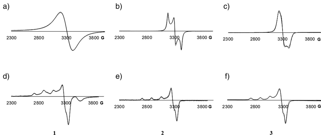
Fig. 4. EPR X-band spectra of complexes 1 (a), 2 (b) and 3 (c) in the solid state ( T=298 K); complex 1 (d) and 2 (e) in phosphate buffer ( T=77 K) and complex 3 (f) in MeOH ( T=77 K). The experimental spectra are presented at light gray and the calculated in black.
