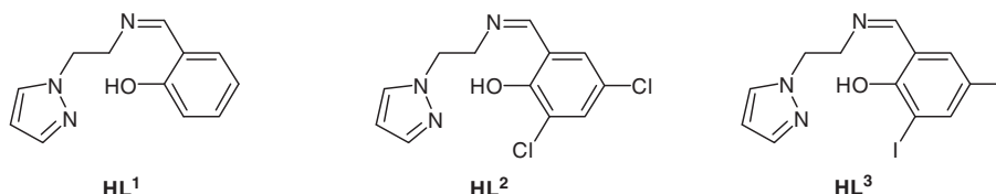
Fig. 1. Tridentate pyrazole-containing ligands of the Schiff base type (L 1 –L 3 ) used to prepare the Cu(II) complexes.
