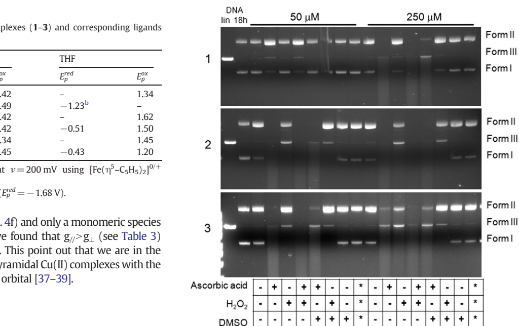
Fig. 6. Cleavage of supercoiled \phi X174 DNA by the Cu(II) complexes ( 1–3 ) after 18 h of incubation at 37 °C in phosphate buffer (pH 7.2), in the presence of reducing or oxidizing agents or in the dark (*). DNA lin – Linear DNA obtained by digestion with Xho I. Forms I, II and III are supercoiled, nicked circular and linear forms of DNA, respectively.
